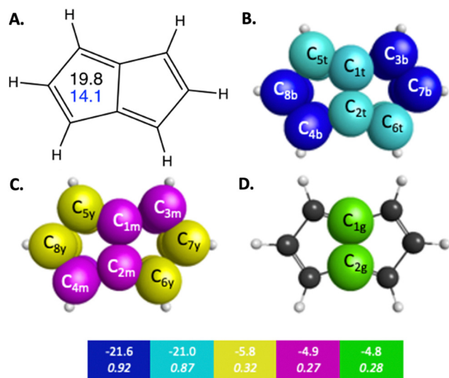
Fig. 2 \pi -Bonding interaction types for pentalene that arise from the symmetry unique QUAOs shown in Fig. S5 (ESI † ). The colored boxes give the KBO ( \text{kcal mol}^{-1} ) with the BO underneath for the corresponding colored \pi -bonding QUAOs. Each set of KBOs with a given color QUAOs have the same bond order. The atom numbers are generated by GAMESS. (A) The numbers inside the pentalene structure in black, and blue correspond to NICS(0) and NICS(1), respectively. (B) Blue = b, and teal = t color labeled QUAOs. (C) Magenta = m, and yellow = y color labeled QUAOs. (D) Green = g color labeled QUAOs.
