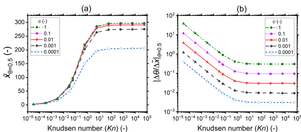
Fig. 11 (a) The penetration depth at half coverage \tilde{x}_{\theta=0.5} and (b) the absolute value of the slope at half coverage |\Delta\theta/\Delta\tilde{x}|_{\theta=0.5} as a function of the Knudsen number for varying sticking coefficients: 1, 0.1, 0.01, 0.001, and 0.0001. The channel height used is 500 nm (the typical PillarHall™ case 17,37 ). To obtain the last four points in the lower Knudsen number regime, a channel height of 1 mm is used, as indicated by the solid triangle symbol. The other parameters used for the simulations are provided in Table 1. The hollow symbols used for data of c = 0.0001 signify the fact that the used exposure did not yet saturate the adsorption at the channel entrance (saturation curves in Fig. S7, ESI†).
