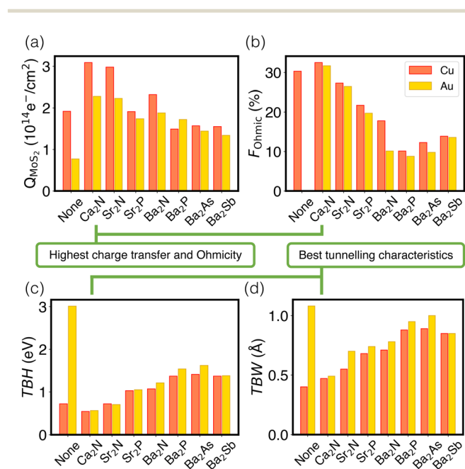
Fig. 4 Bar graphs showing the variation of four figures of merit as a function of the electrene in the metal/electrene/ \text{MoS}_2 contacts. The individual plots show: (a) the charge transfer to \text{MoS}_2 , Q_{\text{MoS}_2} ; (b) the fraction of the contact area that is Ohmic, F_{\text{Ohmic}} ; (c) the tunneling barrier height, TBH; and (d) tunneling barrier width, TBW. Results for the metal/ \text{MoS}_2 interfaces with no electrene are shown for comparison; note that the Q_{\text{MoS}_2} for these two cases results from mid-gap states rather than from the \text{MoS}_2 conduction band.
