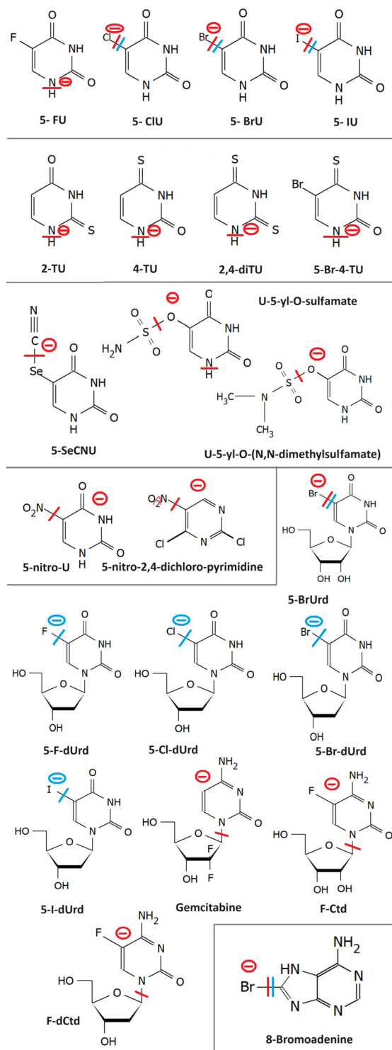
Fig. 3 Radiosensitizers from the group of modified DNA components and their model compounds, whose reactivity with LEES is discussed in the text. From top to bottom halouracils (2.1); 5-selenocyanatouracil (2.3), uracil-5-yl-O-sulfamate and uracil-5-yl-O-(N,N-dimethylsulfamate) (2.4); 5-nitro-uracil (2.5) and 5-nitro-2,4-dichloropyrimidine (2.6); modified nucleosides (2.8) and 8-bromo-adenine (2.7). The red line marks the bond broken in the most intense DEA reaction of the molecule identified for the isolated molecule, and the blue line the dissociation for a solvated molecule. The minus sign marks the anionic DEA fragment.
