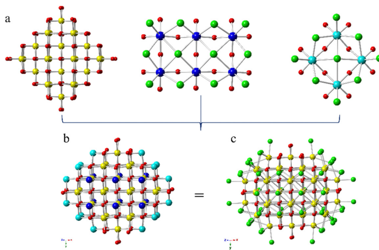
Fig. 1 Ball and stick representation of one of the crystallographically unique Ce52 clusters illustrating (a) the {Ce 24 } (yellow), {Ce 6 } (dark blue) and {Ce 4 } (teal) subunits, and (b) the Ce52 core, with the {Ce 24 }, {Ce 6 }, and {Ce 4 } units highlighted. Cl is in green, and O is in red. The chloride/water decorated Ce52 cluster is shown in (c); all of the Ce sites are rendered as yellow spheres. Hydrogen atoms and disorder have been omitted for clarity.
