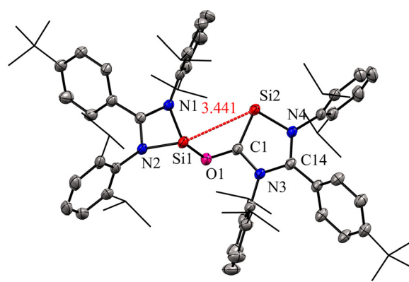
Fig. 4 Molecular structure of 2 showing Si...Si distance between two coordinate and three coordinate Si atoms. Reproduced from ref. 29 ©2022 Wiley–VCH GmbH.
