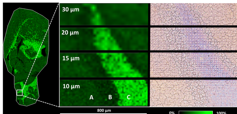
Fig. 3 AgLDI MSI (Ag 6 nm) analysis of cholesterol ( m/z 493.2, [ M + ^{107}\text{Ag}^+ ]). The whole brain section (left) at a spatial resolution of 50 \mu\text{m} . The mouse cerebellum (middle) at spatial resolutions of 30 \mu\text{m} , 20 \mu\text{m} , 15 \mu\text{m} , and 10 \mu\text{m} illustrates the distinct variations in cholesterol intensity between (A) the lobule/molecular layer, (B) the lobule/granular layer, and (C) fiber tracks. An optical microscope image (right) of the mouse cerebellum shows the section after analysis with laser ablation spots.
