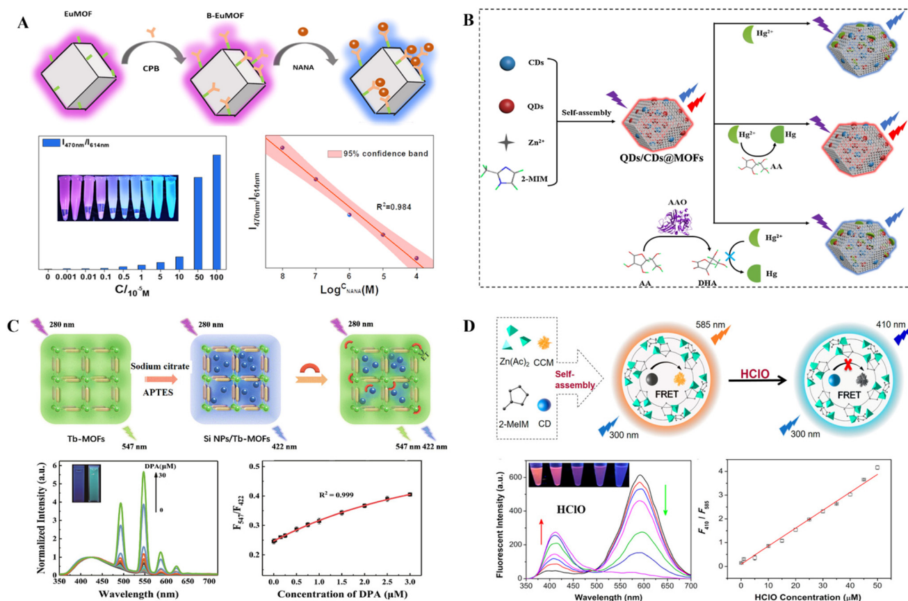
Fig. 9 Biomarker sensing of MOF-based ratiometric fluorescent probes. (A) Schematic representation of the dual emission B-Eu-MOF probe for NANA detection and the relationship of I_{470\text{ nm}}/I_{614\text{ nm}} with different concentrations of NANA. 88 (B) Schematic representation of the synthesis of dual-emission QDs/CDs@MOFs and the ratiometric fluorescence sensing of AA and AAO. 89 (C) Schematic description of the preparation of Si NPs/Tb-MOFs and sensing process towards DPA. 90 (D) Schematic diagram of the synthesis of dual-emission CD/CCM@ZIF-8 and ratiometric fluorescence detection of HClO. 91
