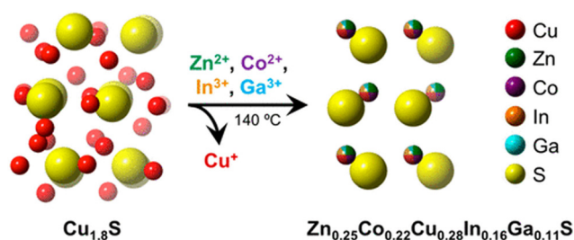
Fig. 2 Figure visually showing the formation of (\text{Zn}_{0.25}\text{Co}_{0.22}\text{Cu}_{0.28}\text{In}_{0.16}\text{Ga}_{0.11})\text{S} HE metal sulfide synthesis via simultaneous multication exchange. Copyright permission from American Chemical Society, used from ref. 65.
