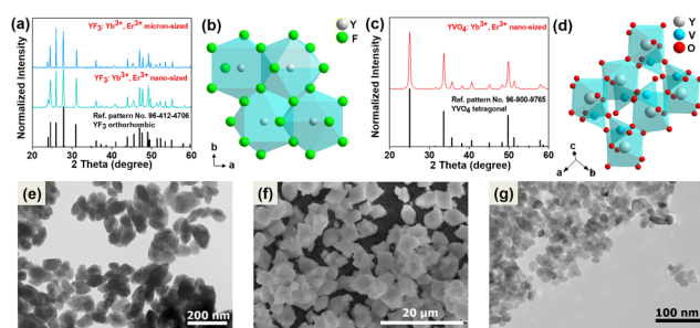
Fig. 1 Powder XRD patterns of the (a) \text{YF}_3:20\% \text{Yb}^{3+}, 2\% \text{Er}^{3+} and (c) \text{YVO}_4:20\% \text{Yb}^{3+}, 2\% \text{Er}^{3+} and (b and d) corresponding graphical representation of the arrangement of atoms in the crystal lattice, TEM/SEM images of (e) nanocrystalline \text{YF}_3:\text{Yb}^{3+}, \text{Er}^{3+} , (f) microcrystalline \text{YF}_3:\text{Yb}^{3+}, \text{Er}^{3+} , and (g) nanocrystalline \text{YVO}_4:\text{Yb}^{3+}, \text{Er}^{3+} .
