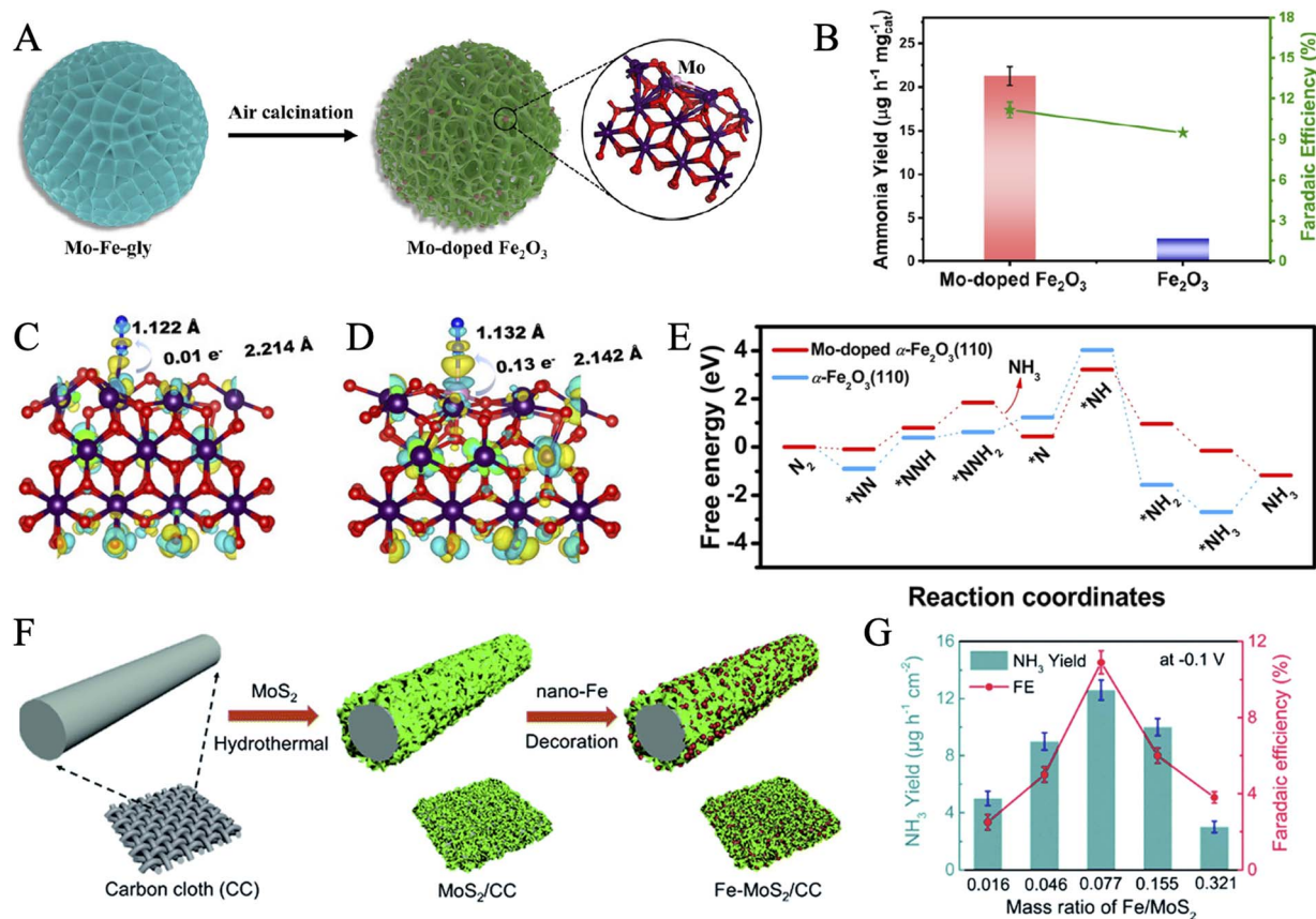
Fig. 7 (A) Diagrammatic representation of the formation of Mo-doped Fe 2 O 3 porous nanospheres. (B) Comparison of NH 3 production rates and FEs at -0.6 V for Mo-doped Fe 2 O 3 and Fe 2 O 3 . The charge density difference of N 2 -adsorbed α-Fe 2 O 3 (110) (C) and Mo-doped α-Fe 2 O 3 (110) (D) with an isosurface value of 0.006 e - Å -3 . (E) Free energy diagram for the NRR process on α-Fe 2 O 3 (110) and Mo-doped α-Fe 2 O 3 (110), respectively. Reproduced with permission: copyright 2022, American Chemical Society. 143 (F) Schematic illustration for the formation routes of Fe-MoS 2 /CC. (G) NH 3 yield and FE with different mass ratios of Fe-MoS 2 . Loading mass: 2.15 mg cm -2 . Reproduced with permission: copyright 2019, Royal Society of Chemistry. 152
