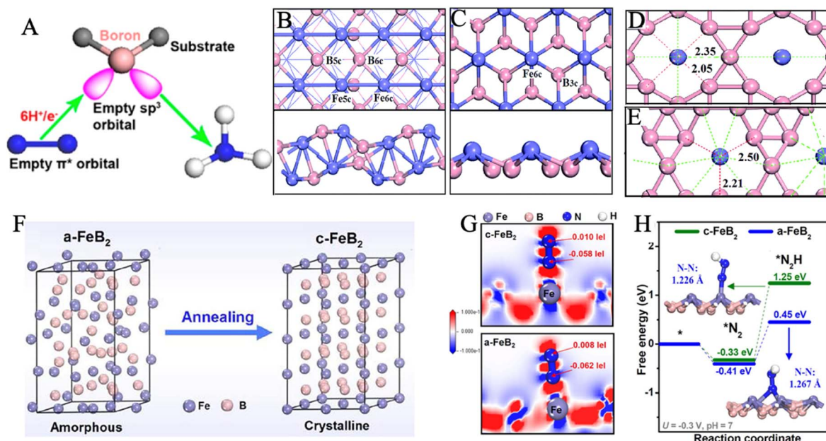
Fig. 11 (A) Schematic of \pi -backdonation between boron and \text{N}_2 . Reproduced with permission: copyright 2019, American Chemical Society. 192 Top and side views of FeB (B) and FeB 2 (C). Fe and B are represented as purple and pink balls, respectively. Models and bonding network for (D) FeB 6 ( \alpha ) and (E) FeB 6 ( \beta ). The length of Fe–B 5c (short) and Fe–B 6c (long) bonds are labeled in units of Å. Reproduced with permission: copyright 2019, Royal Society of Chemistry. 58 (F) Illustration of the phase transformation from a-FeB 2 to c-FeB 2 . (G) Charge density difference: the electron accumulation and depletion are represented as red and blue regions, respectively. (H) Free energy profiles of *N 2 and *N 2 H adsorption on c-FeB 2 and a-FeB 2 . Reproduced with permission: copyright 2021, Elsevier. 57
