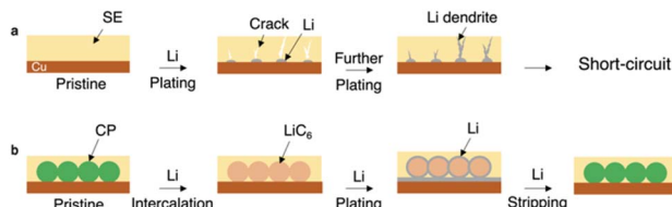
Fig. 1 Schematic diagrams of different current collectors for AFSSLBs. (a) Lithium nuclei are formed on the surface of Cu. Volumetric changes during the Li plating process can easily break the SE, especially at high areal capacity. This behavior leads to the growth of cracks and subsequent Li dendrites, which results in short-circuit. (b) The modification of the Cu substrate with an interconnected carbon paper creates a host with large plating sites for stabilizing the lithium intercalation and the subsequent plating. The volumetric change of the Li plating is accommodated by the flexible interconnected carbon paper.
