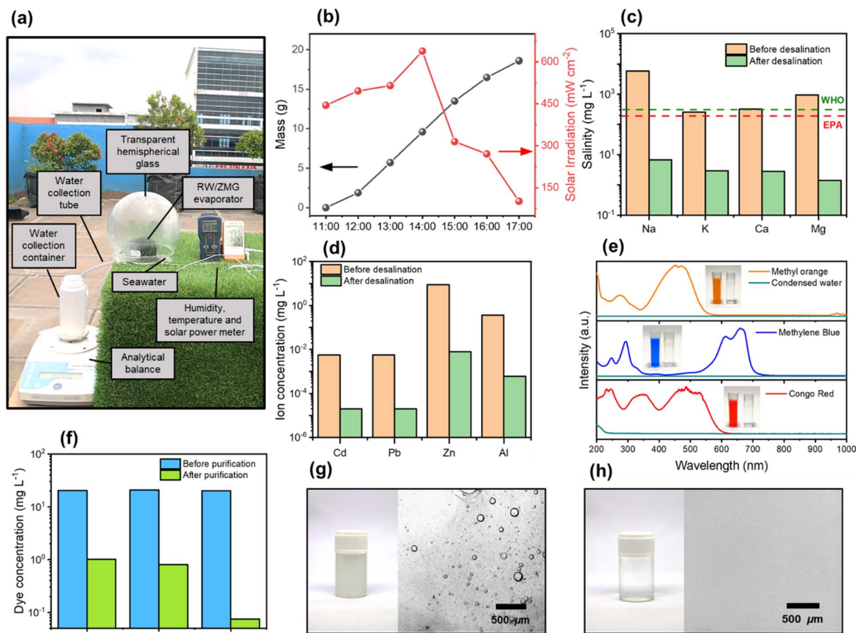
Fig. 7 (a) Photograph of outdoor water evaporation experiment prototypes with sealed dome-type chambers, (b) mass of water collected on evaporator ( 6 \times 6 cm 2 ) under natural sunlight. (c) The concentration of four kind of primary ions (Na + , K + , Ca 2+ and Mg 2+ ), (d) heavy metal ions (Cd 2+ , Pb 2+ , Zn 2+ and Al 3+ ) of before and after desalination from domestic wastewater, (e) UV-Vis spectra of MO, MB and CR organic dyes solution and (f) removal performance before and after purification. (g) Micrographs and optical microscope photos of oil/water emulsion before and (h) after purification.
