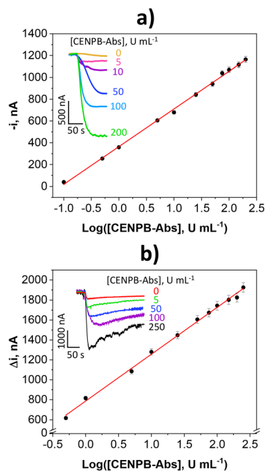
Fig. 2 Calibration plots and amperometric traces (inset) provided by the MB-assisted a) and integrated b) immunoplateforms for the determination of CENPB-Abs standards.
