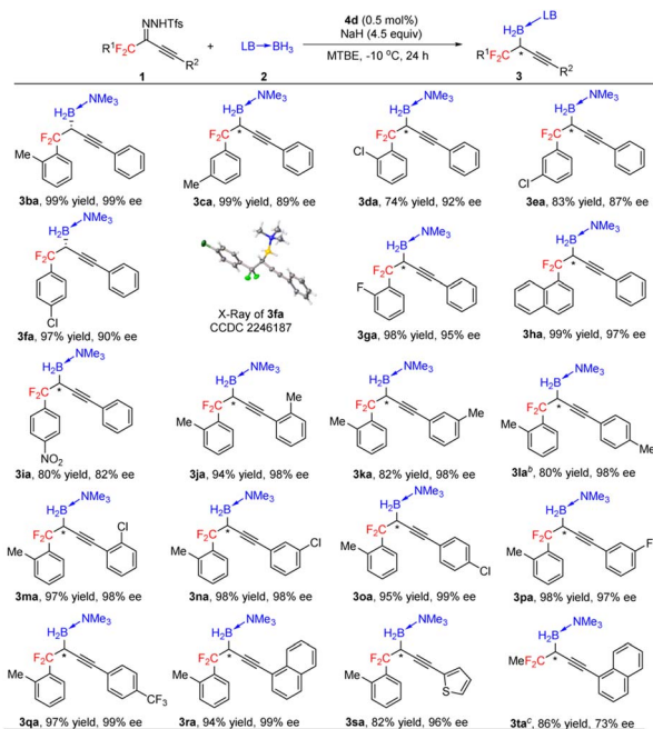
Scheme 3 Preparation of chiral gem -difluoroalkyl \alpha -allenols through addition reactions of gem -difluoroalkyl propargylic boron with aldehydes. a ( \text{CH}_2\text{O} ) n (10 equiv.).
