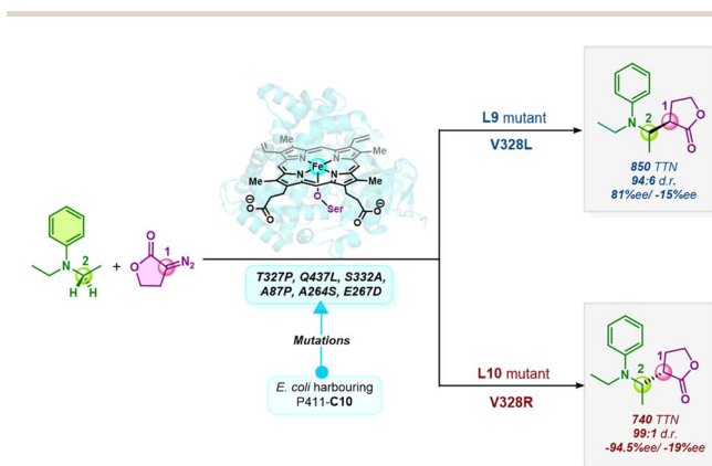
Scheme 1 Enzymatic enantiodivergent C(sp 3 )-H insertion catalyzed by ‘P411’ mutants. Further mutations resulted in two mutants, L9 and L10, differing by a single point mutation (V328L/R), showing opposite stereopreference for this C-H insertion reaction ( 1 and 2 denote the two chiral centers on the carbene C and the secondary C center of aniline, respectively).
