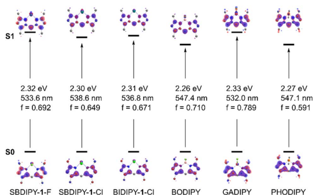
Fig. 4 Computed first electronic transition of different dipyrin derivatives at the CPCM-SCS-CIS(D)/def2-TZVPP// r^2 SCAN-3c level. The Natural Transition Orbitals involved in the main \pi \rightarrow \pi^* excitations are displayed together with the predicted energies and oscillator strengths.
