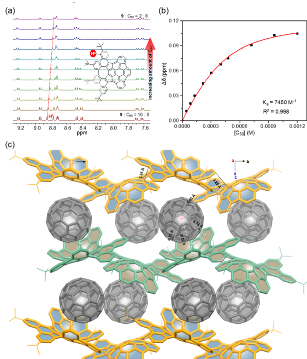
Fig. 7 (a) Selected regions of 1 H NMR spectra during titration of 9 with C 60 (the total concentration [9] + [C 60 ] = 6.0 × 10 -4 M, toluene- d 8 , 298 K); (b) fitting curves for the proton H A in 9 vs. [C 60 ]; (c) crystal packing of 9·C 60 with selected centroid–centroid distances and close contact distances (Å).
