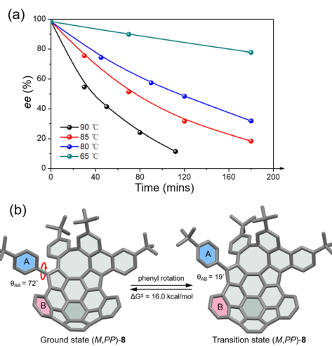
Fig. 4 (a) Racemization kinetic plots of enantiomerized 9 in toluene at various temperatures; (b) the rotation process and rotation barrier of the pendant phenyl ring in ( M,PP )- 8 at the B3LYP/6-311G(d,p) level.
