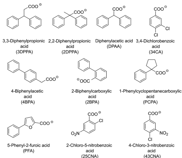
Fig. 2 Carboxylate anions utilized in the solubility screening.
