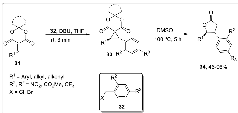
Scheme 12 Synthesis of substituted trans -β,γ-disubstituted-γ-butyrolactones 34 via Cloke–Wilson rearrangement.
