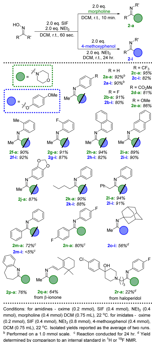
Fig. 2 Substrate scope for the conversion of ketoximes to amidine and imide products via SIF reagents.
