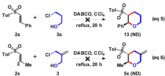
Scheme 6 Unsuccessful reactions.
