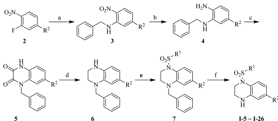
Scheme 2 Reagents and conditions: (a) benzylamine, K 2 CO 3 , MeCN, reflux, 1.5 h; (b) 10% Pd/C, H 2 , MeOH, rt, 2 h; (c) diethyl oxalate, 140 °C, 4 h; (d) BH 3 –THF, anhydrous THF, 0 °C, 30 min then rt, 12 h; (e) corresponding sulfonyl chloride, DMAP (cat.), TEA, anhydrous DCM, rt, 2 h; (f) Raney Ni, H 2 , MeOH, 60 °C, 4 h.
