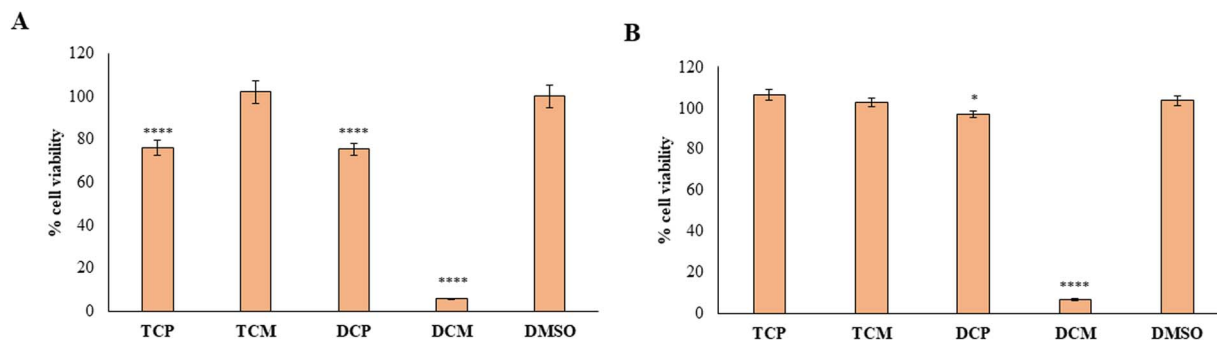
Fig. 8 MTT test on AGS treated with the hit compounds. MTT test on AGS treated with TCP, TCM, DCP and DCM at 50 μM for 48 h (A) and 72 h (B); DMSO: control vehicle. Data are presented as mean% ± SD. The most representative of three different experiment is shown. (A) **** vs. DMSO p < 0.0001 ; (B) * vs. DMSO p = 0.0172 , **** vs. DMSO p < 0.0001 .
