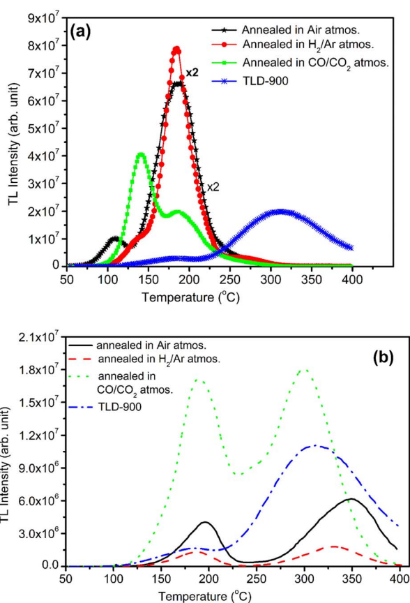
Fig. 13 (a) Comparison of TL sensitivity of the NaLi 2 PO 4 :Cu(II) materials annealed in air, in 10% H 2 in Ar and in CO/CO 2 atmospheres annealed at 400, 600 and 800 °C, respectively, with that of CaSO 4 :Dy (TLD-900) phosphor, (b) similar comparison of NaLi 2 PO 4 :Cu(II) phosphors annealed under same conditions.
