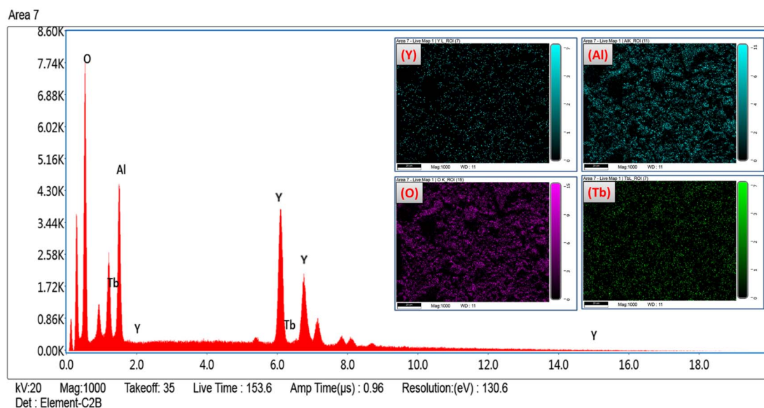
Fig. 7 EDX spectral profile of optimized \text{Y}_{3.97}\text{Al}_2\text{O}_9:0.03\text{Tb}^{3+} phosphors and inset represent the field view corresponding to each atoms present in \text{Y}_{3.97}\text{Al}_2\text{O}_9:0.03\text{Tb}^{3+} sample.
