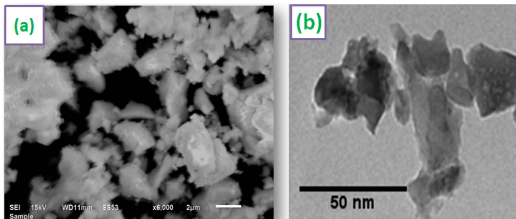
Fig. 6 Micrographs (a) SEM (b) TEM of optimized \text{Y}_{3.97}\text{Al}_2\text{O}_9:0.03\text{Tb}^{3+} sample.
