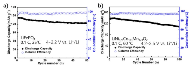
Fig. 5 Cyclic performance of \text{LiFePO}_4 /PA2-PEO-10% LLZO/Li cells at 0.1C, 25 °C, and NCM111/PA2-PEO-10% LLZO/Li cells at 0.1C, 60 °C.
