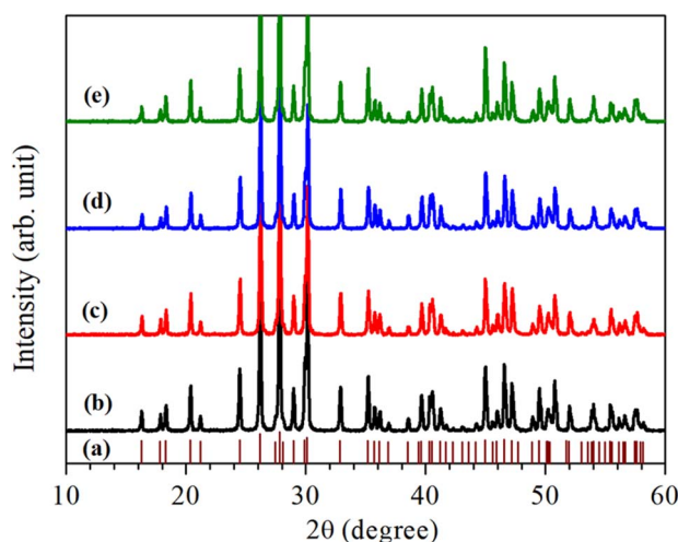
Fig. 1 Room-temperature XRD patterns of \text{Eu}^{3+} and/or \text{Cr}^{3+} co-doped \text{LaVO}_4 phosphors: (a) Standard XRD pattern of \text{LaVO}_4 (JCPDF File No. 50-0367), (b) \text{LaVO}_4\cdot 1\text{Eu}^{3+} , (c) \text{LaVO}_4\cdot 1\text{Eu}^{3+}\cdot 0.01\text{Cr}^{3+} , (d) \text{LaVO}_4\cdot 1\text{Eu}^{3+}\cdot 0.05\text{Cr}^{3+} and (e) \text{LaVO}_4\cdot 1\text{Eu}^{3+}\cdot 0.1\text{Cr}^{3+} phosphors.
