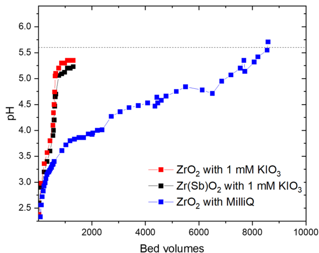
Fig. 2 pH of eluate in \text{ZrO}_2 with 1 mM \text{KIO}_3 (red squares), \text{Zr}(\text{Sb})\text{O}_2 with 1 mM \text{KIO}_3 (black squares) and \text{ZrO}_2 with deionized water (blue squares). The pH of the feed was 5.6 and is shown as dashed horizontal line. The uncertainty of individual pH measurement was estimated to be 0.1 units.
