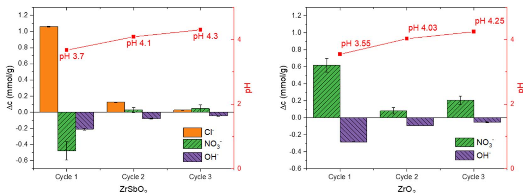
Fig. 1 Anions adsorbed and desorbed during successive equilibrations of \text{Zr}(\text{Sb})\text{O}_2 and \text{ZrO}_2 with 10 mM \text{NaNO}_3 (pH 5.6). The negative values represent adsorption to the material and the positive values represent desorption to the solution phase. The standard deviations of pH measurements are now showing in figure as they were extremely small related to the measured value.
