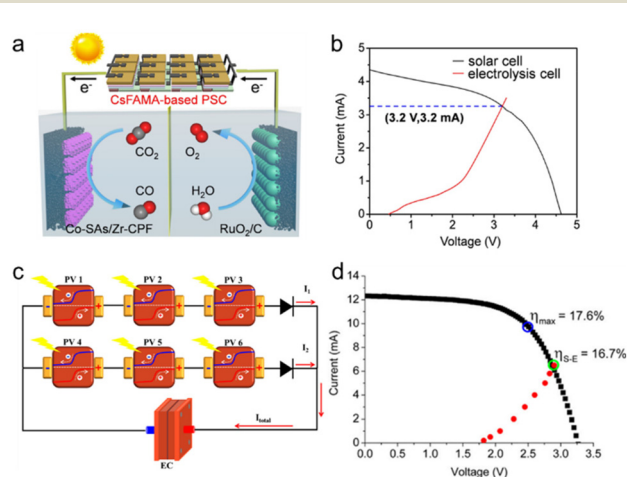
Fig. 12 Halide perovskite PV-EC devices for solar hydrocarbon generation. (a) Schematic illustration of the integrated solar-driven CRR-OER electrolysis system powered by a homemade large-area CsFAMA-based perovskite solar cell. (b) J - V curves for large-area CsFAMA-based perovskite solar cell- \text{RuO}_2/\text{C} anode//Co-SAs/Zr-CPF cathode. Reproduced from ref. 199. Copyright 2022 American Chemical Society. (c) Schematic diagram of the perovskite module connected to the electrolyzer. (d) J - V characteristic of the perovskite minimodule and measured operating current of the electrolyzer. Reproduced from ref. 200. Copyright 2019 PNAS.
