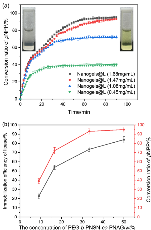
Fig. 8 (a) Catalytic hydrolysis process of p NPP by the nanogels with various concentrations. (b) Immobilization efficiency of lipase versus the concentration of the polymers.
