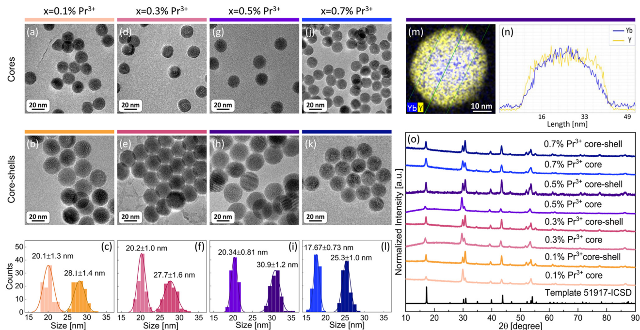
Fig. 1 Characteristic of \beta -NaYF 4 nanocrystals co-doped with x\% \text{Pr}^{3+} and 15% \text{Yb}^{3+} ions showing PA: (a, d, g and j) transmission electron microscopy (TEM) images of core nanoparticles; (b, e, h and k) TEM images of core-shell nanocrystals; (c, f, i and l) histograms with average sizes of core and core-shell nanocrystals. (m) Energy dispersive X-ray spectroscopy (EDS) map and (n) EDS profile of \text{Yb}^{3+} and \text{Y}^{3+} ions in the core-shell NaYF 4 :0.5% \text{Pr}^{3+} , 15% \text{Yb}^{3+} @NaYF 4 nanocrystals; (o) X-ray powder diffractions of the \beta -NaYF 4 structure (template) and all the samples.
