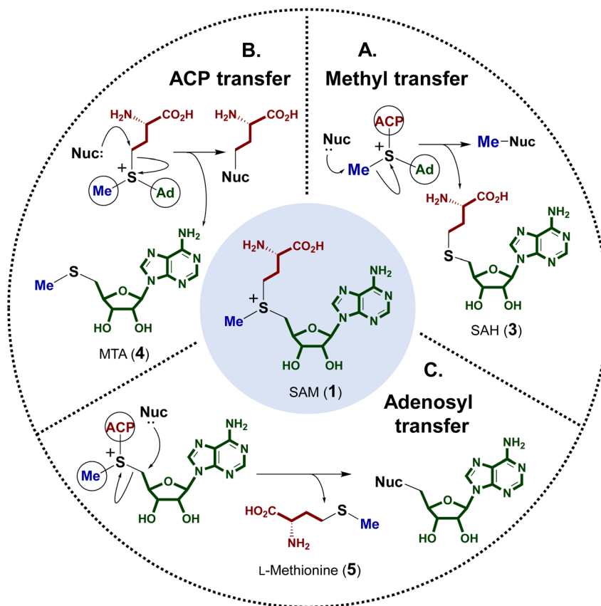
Fig. 2 Summary of SAM-dependent alkylation reactions, showing the by-product generated following each group transfer. (A) Methyl transfer yields S-adenosyl homocysteine (SAH, 3), (B) ACP (3-amino-3-carboxypropyl) transfer yields 5'-methylthioladenosine (MTA, 4) and (C) adenosyl transfer yields L-methionine (5).
