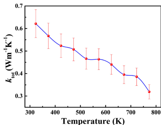
Fig. 5 The temperature-dependent total thermal conductivity ( k_{\text{tot}} ) for the polycrystalline sample of \text{BaCeCuS}_3 .
