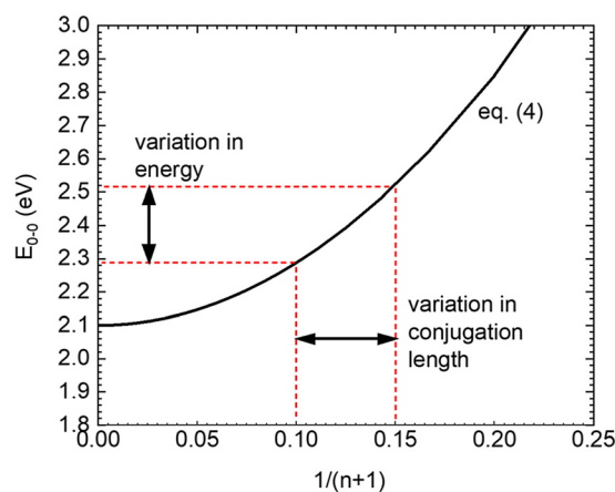
Fig. 6 Illustration on the relation between the variations of conjugation length and transition energy on the basis of eqn (4). n denotes the number of double bonds, E_{0-0} is the energy of the first excited singlet state. The values are parametrized to describe PDOPT.
