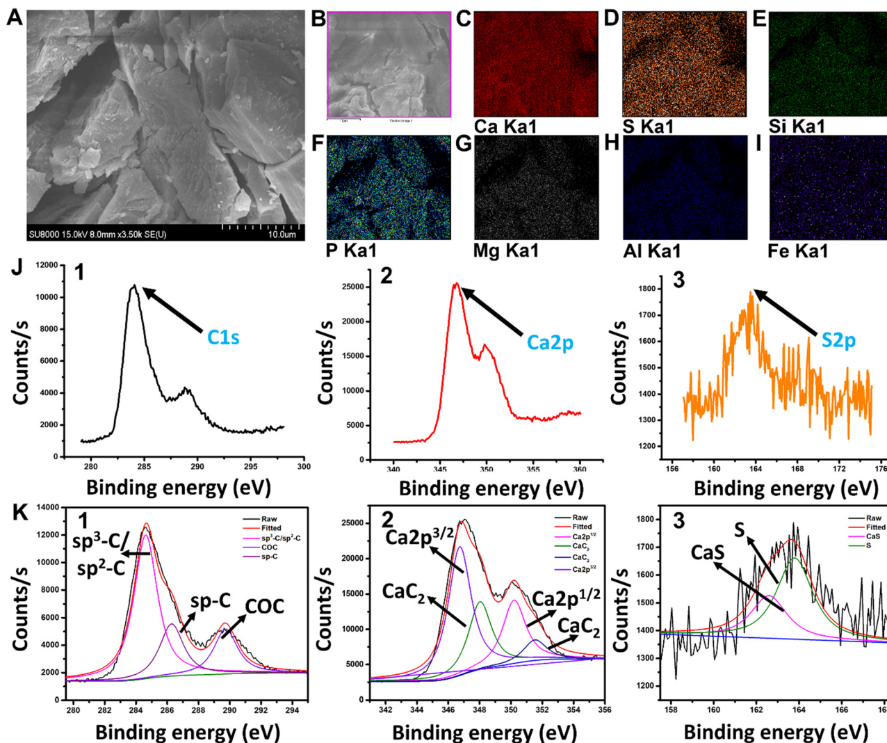
Fig. 1 (A) SEM image of \text{CaC}_2 at 10 \mu\text{m} . (B)–(I) Distribution of all elements and their core-level studies based on SEM mapping. (J1–3) XPS data. (K1–3) Fitted XPS data for carbon, calcium, and sulfur distribution.
