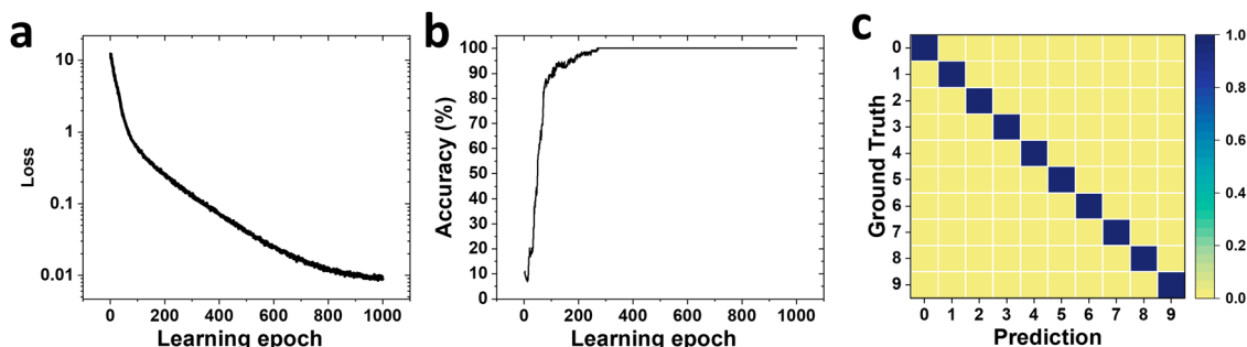
Fig. 6 Training and performance evaluation of the SiC memristor-based reservoir computing system. (a) The training loss as a function of learning epochs. (b) The validation accuracy as the function of learning epochs. (c) Confusion matrix showing the prediction results from the RC system against the ground truth in the test dataset.
