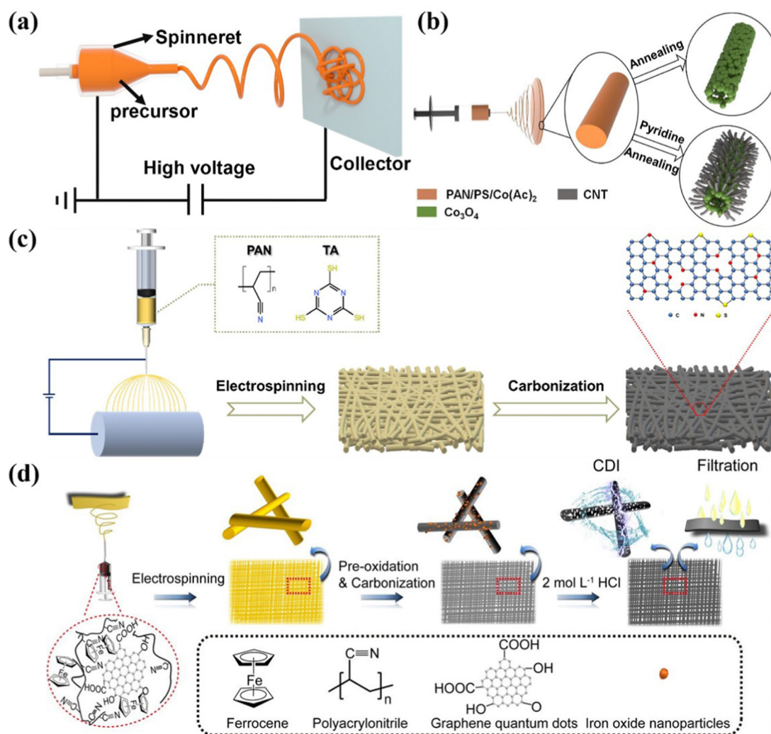
Fig. 3 (a) Schematic diagrams of the electrospinning process. Illustration of the preparation of the freestanding (b) \text{Co}_3\text{O}_4 @CNF@CNT and (c) S/N co-doped CNT electrodes, reproduced from ref. 88 and 89 with permission from Elsevier. (d) Schematic of the fabrication of graphene quantum dot modified CNT electrodes, reproduced from ref. 90 with permission from the American Chemical Society.
