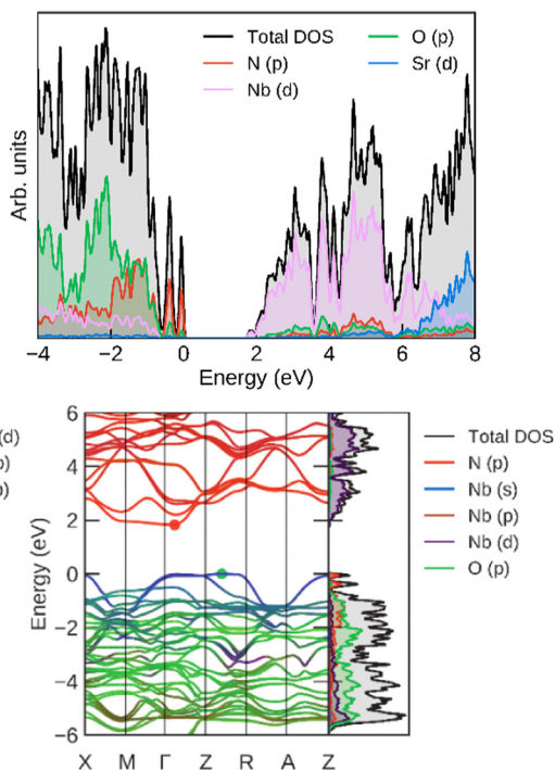
Fig. 12 (left) Total and projected densities of states and (right) band structure for SrNbO 2 N, calculated at the HSE06 level.
