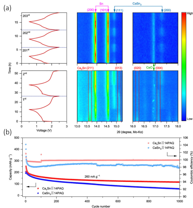
Fig. 8 (a) Isoplots of in situ XRD scans the anode Ca x Sn n ||14PAQ cells during the first, second and from 201st to 203rd discharge/charge cycles at specific current of 26 mA g -1 at 25 °C. The peak is observed along the top and the cell voltage profiles on the left had side. ICSD-ID: Ca 2 Sn 659 611, β-Sn 106 072, CaSn 3 58 934, Ca 36 Sn 23 54 619 and CaO 26 959. (b) Cycling performance of CaSn 3 ||14PAQ compared with Ca x Sn||14PAQ. Reproduced with permission from ref. 94, copyright 2022 Springer Nature.
