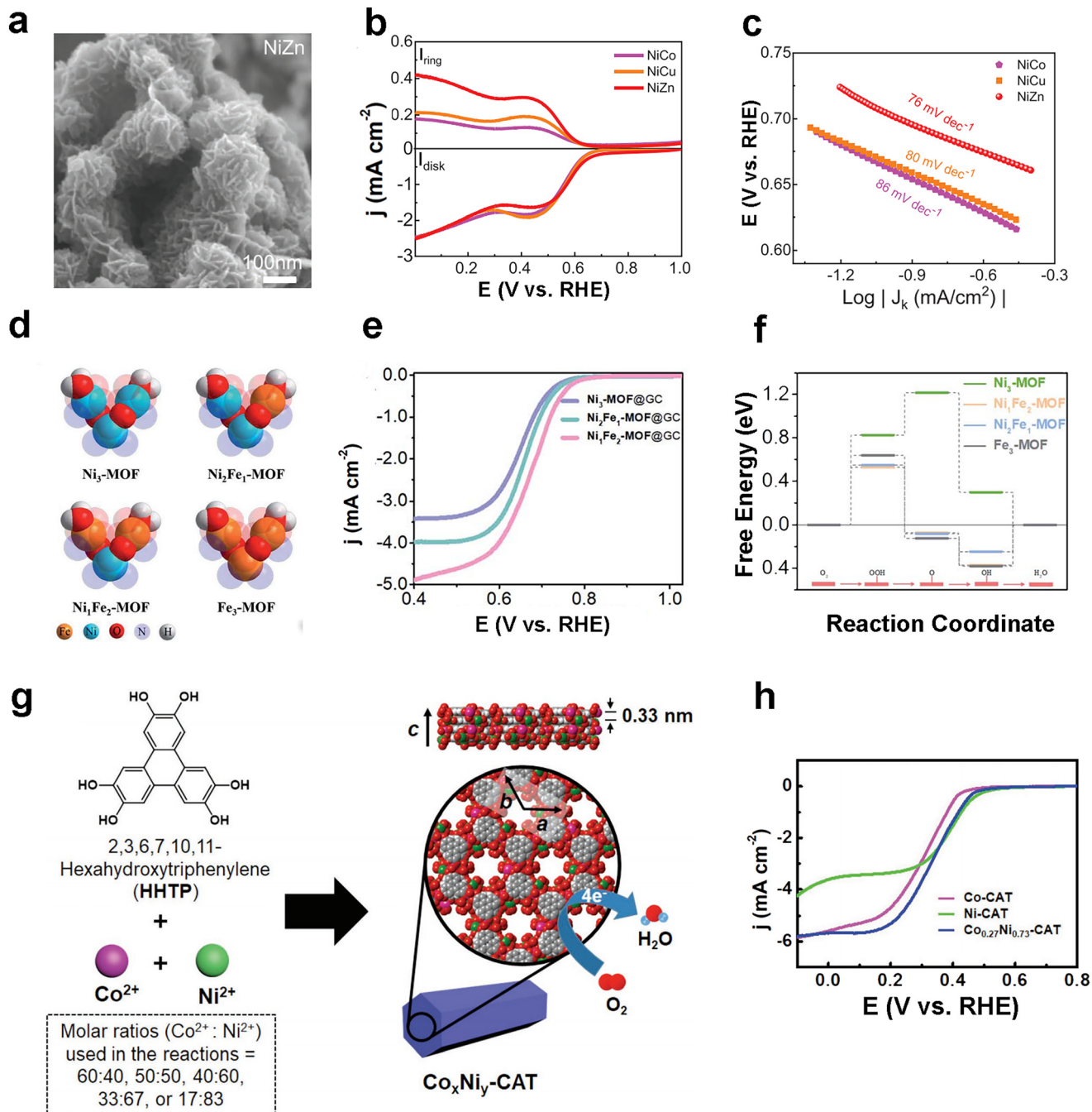
Fig. 9 MOF-based ORR electrocatalysts. (a) SEM images of NiZn MOF; (b) LSV curves and (c) Tafel slope of NiM MOF for ORR tests in \text{O}_2 -saturated 0.1 \text{ M KOH} . Rotation rate: 1600 \text{ rpm} . Reproduced with permission. 90 Copyright 2022, Wiley-VCH; (d) visual representation of the established V-shaped trinuclear clusters; (e) LSV curves of \text{Ni}_1\text{Fe}_2\text{-MOF@GC} and other samples for ORR tests in \text{O}_2 -saturated 0.1 \text{ M KOH} , rotation rate: 2500 \text{ rpm} ; (f) calculated free energy diagram of the ORR of \text{Ni}_1\text{Fe}_2\text{-MOF} and other samples at 1.23 \text{ V} . Reproduced with permission. 91 Copyright 2021, The Royal Society of Chemistry; (g) schematic diagram of the construction of bimetallic 2D MOF \text{Co}_x\text{Ni}_y\text{-CATs} for the ORR; (h) LSV curves of \text{Co}_{0.27}\text{Ni}_{0.73}\text{-CAT} and other samples for ORR tests in \text{O}_2 -saturated 0.1 \text{ M NaClO}_4 and 0.02 \text{ M PBS} , rotation rate: 1600 \text{ rpm} . Reproduced with permission. 92 Copyright 2019, Wiley-VCH.
