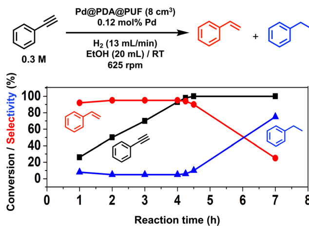
Fig. 5 Hydrogenation of phenylacetylene with Pd@PDA@PUF ( 8 \text{ cm}^3 ); 0.12 mol% Pd; black squares: PA conversion; red circles, ST selectivity; blue triangles: EB selectivity. Reaction conditions: PA ( 6 \text{ mmol} ), Pd ( 7 \times 10^{-3} \text{ mmol} ), EtOH (20 mL), \text{H}_2 flow rate ( 13 \text{ mL min}^{-1} ), room temperature, 625 rpm.
