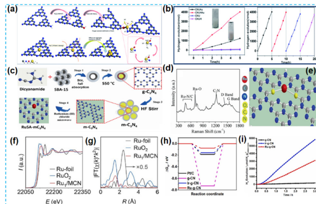
Fig. 12 (a) Schematic of the structural evolution of CNUHAu. (b) Photocatalytic hydrogen evolution activity over CNUAu and CNUHAu under visible light irradiation. 61 (c) Schematic representation of the synthesis protocol for ruthenium single atom over mesoporous C 3 N 4 . (d) Raman spectra of RuSA-mC 3 N 4 . (e) Schematic illustration of the Ru coordination with nitrogen in the CN matrix of the RuSA-mC 3 N 4 photocatalyst. 62 (f) Ru K-edge XANES spectrum. (g) FT-EXAFS spectrum. 63 (h) The Gibbs free-energy diagram towards the HER of the pristine g-CN, Ir-g-CN, and Ru-g-CN catalysts. (i) Photocatalytic H 2 evolution tests of pristine g-CN, Ir-g-CN and Ru-g-CN catalysts. 64
