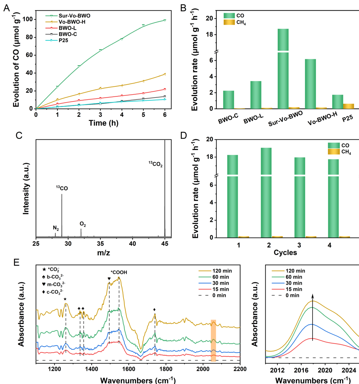
Fig. 3 (A) Time courses of photocatalytic CO evolution curves and (B) CO and CH 4 evolution rate of Sur-Vo-BWO and control samples; (C) mass spectrum of ^{13}\text{CO} produced over Sur-Vo-BWO by a ^{13}\text{CO}_2 isotope labelling experiment; (D) CO and CH 4 evolution rate of Sur-Vo-BWO under stability test; (E) the in situ FTIR study of Sur-Vo-BWO.
