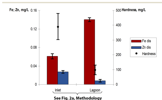
Fig. 7 Metals and water hardness profile during dry weather Fe dis is 0.14 mg L -1 in the lagoon, comprising almost 50% of its total form (Fe tot is 0.29 mg L -1 ).
