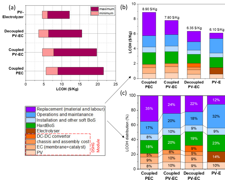
Fig. 2 (a) Range of levelized cost of hydrogen (LCOH) for all direct solar hydrogen generation (DSHG) systems and PV-Electrolyzer for range of component costs, given in Table S3 and S4 in the ESI, † (b) LCOH for all DSHG systems and PV-Electrolyzer for baseline costs with cost breakdown and (c) percentage contribution of different components, divided into module cost (PV, EC, chassis and assembly, dc-dc convertor, electrolyser), hard BoS, soft BoS, operations and maintenance (O&M) and replacement (material and labour) costs.
