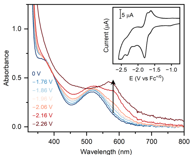
Fig. 10 UV-Vis spectroelectrochemical data for Re5 (1 mM), showing the steady-state relative absorbance at different applied potentials under N_2 . The inset shows the cyclic voltammogram of Re5 at the reductive potential.
