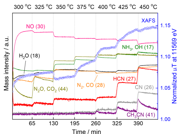
Fig. 4 Changes of the MS spectra and the XAFS intensity (at 11569 eV) at various temperatures raising from 300 to 450 °C with 25 °C steps. Reaction conditions: 5 wt% \text{Pt}/\text{Al}_2\text{O}_3 (100 mg), \text{CH}_4 : \text{NO} : \text{He} = 13.4 :1.8:84.8 (total flow rate: 100 \text{mL min}^{-1} ), and 0.1 MPa.
