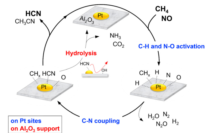
Scheme 2 Proposed steps for the reaction of \text{CH}_4 and \text{NO} on \text{Pt}/\text{Al}_2\text{O}_3 catalysts.
